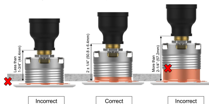
Figure 7: Installation (Correct and Incorrect)
