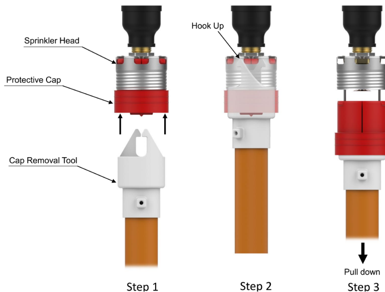
Figure 5: Protective Cap Removal
