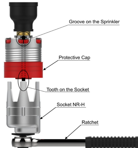
Figure 4: Ratchet & Socket
