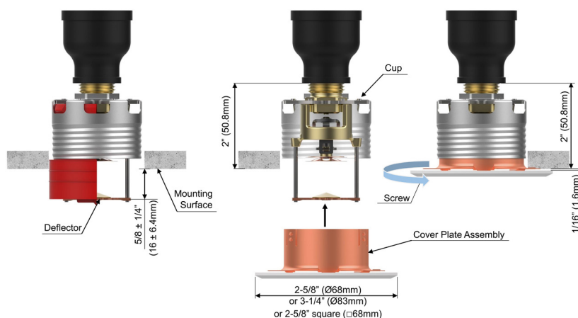
Figure 6: Installation (Cover Plate Assembly)
